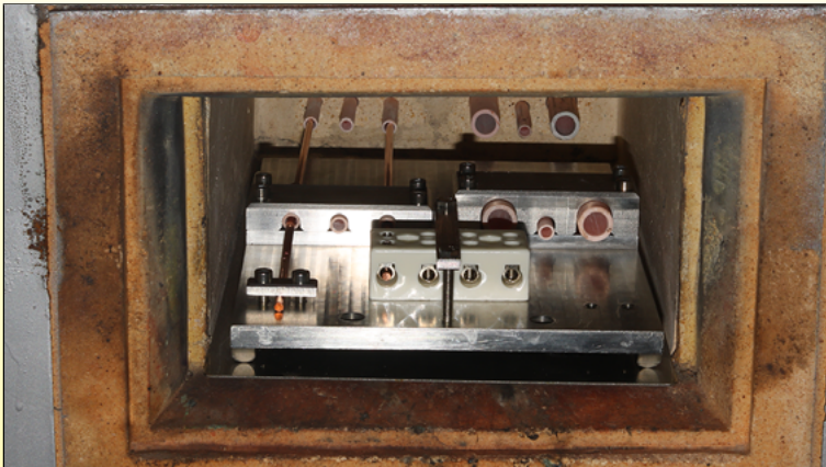
Test oven for the resistivity of ceramics as a function of temperature (Ultimheat Laboratory)
