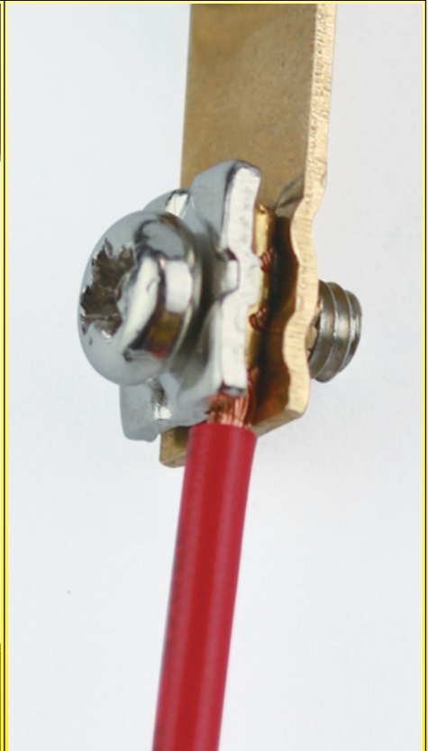
Terminal detail
